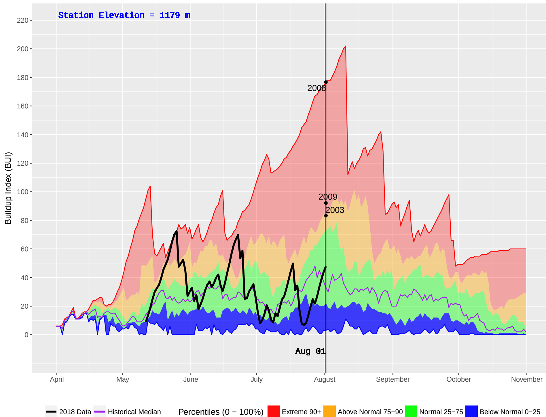
HOLMES (201) : Historical (1987–2016) and Current (2018) Daily Buildup Index (BUI)
